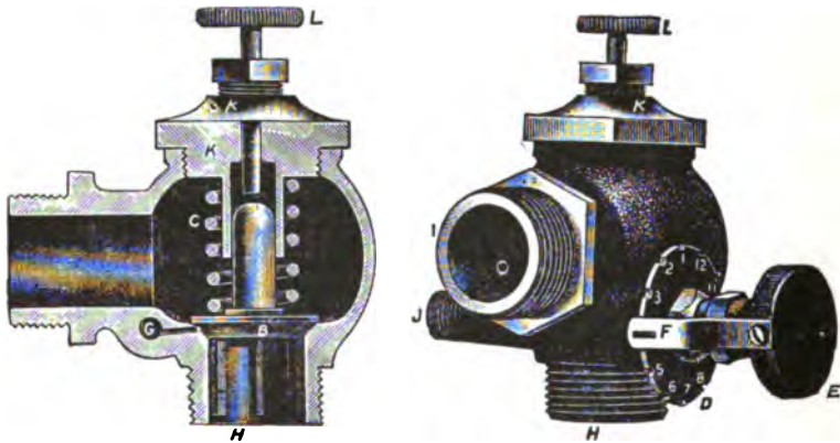
FIG. 319.—The James Valve. B, fuel inlet valve; C, spring controlling B; D is the scale dial showing proportions of air and gasoline; E, the wheel controlling gasoline valve; F, clip or top for holding E in position; G, gasoline supply tube; H, air inlet; I, entrance to cylinder; J, entrance for gasoline; K, cover of valve chamber; L, wheel and spindle controlling tension of spring, C.
